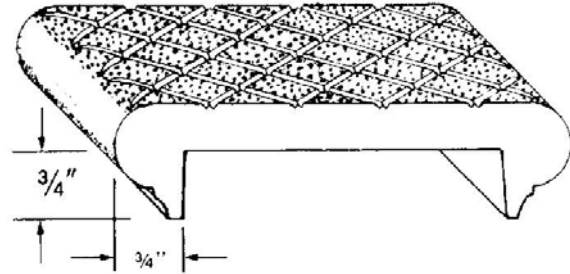
TYPE 106A Double Nose – 3/4" x 3/4" DRAWING NOT TO SCALE
