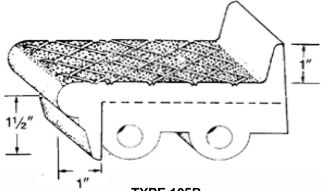
TYPE 105B Nose – 1" x 1 1/2" Toeplate 1" DRAWING NOT TO SCALE
