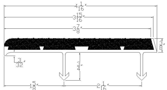
Type WP4J
