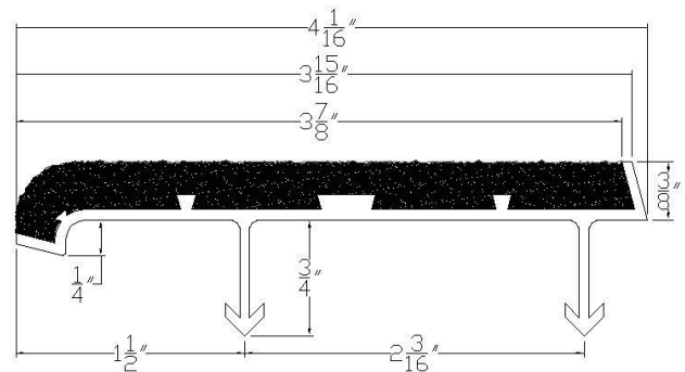
4 1/16" wide, 3/8" thick, nose 1/4" underside DRAWING NOT TO SCALE Maximum length is 10'-0".
