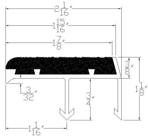
2 1/16" wide, 3/8" thick DRAWING NOT TO SCALE Maximum length is 10'-0".
