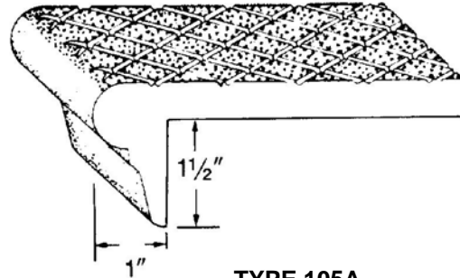
TYPE 105A Nose – 1" x 1 1/2" DRAWING NOT TO SCALE
