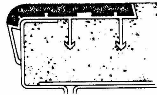
Detail - sure hold anchor in steel pan step
