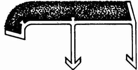
Type WP2C 2 1/16" wide, 3/8" thick, nose 1/4" underside DRAWING NOT TO SCALE
