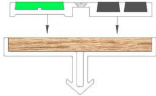
TYPE 630B-NG 3 7/32" wide, 3/8" thick DRAWING NOT TO SCALE
