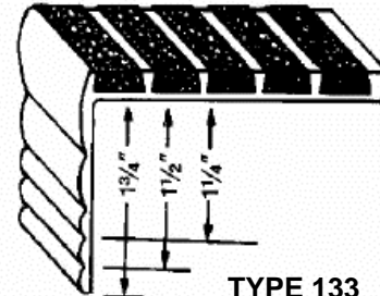
TYPE 133 HAS VARIABLE NOSE DEPTH 3" wide, 1/4" thick, nose 1 3/4" underside Nose can be sheared for additional charge DRAWING NOT TO SCALE
