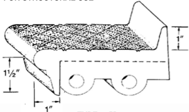
TYPE 105B Nose – 1" x 1 1/2" Toeplate 1" DRAWING NOT TO SCALE
