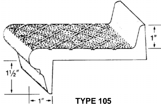
TYPE 105 Nose – 1" x 1 1/2" Toeplate 1" DRAWING NOT TO SCALE
